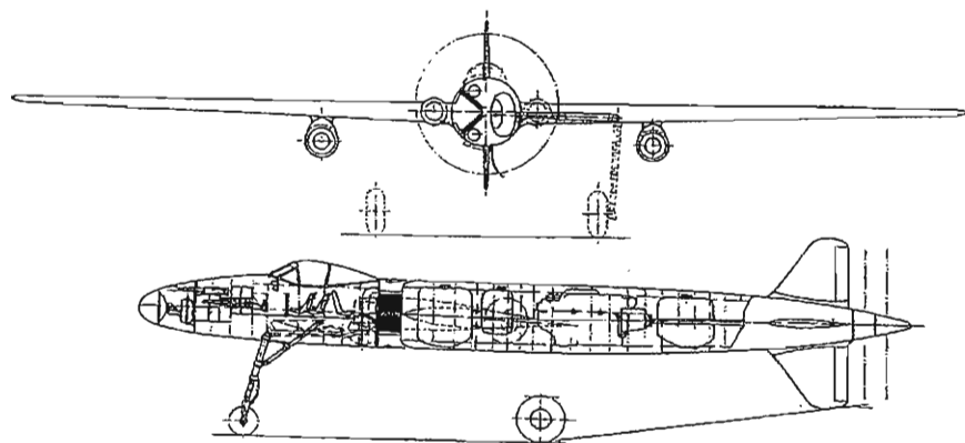
Focke-Wulf 0310251-13 Night and Bad-weather Fighter. This variant drove contraprops and had short wingroot air intakes.
