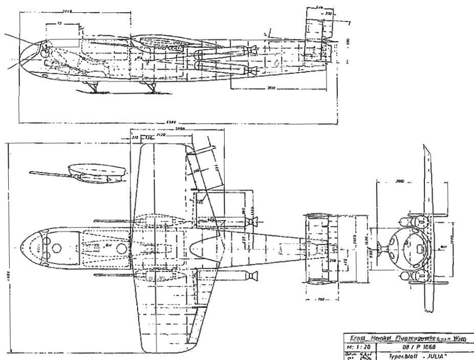
Heinkel P1077 'Julia I' with prone pilot and four RATO units.
