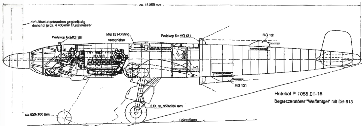
Heinkel P1055.01-16 sectional side-view.
