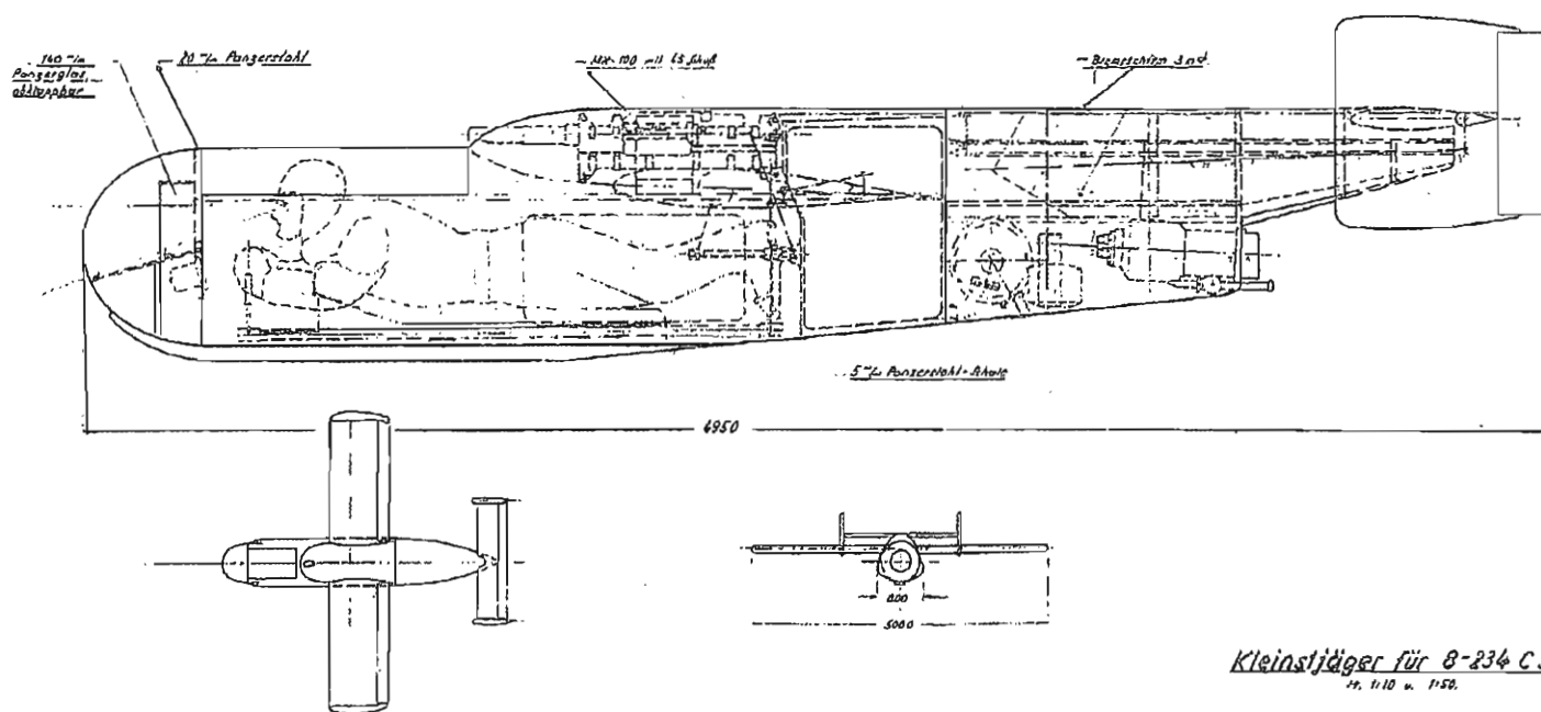
Arado E 381 three-view works drawing of 1st December 1944. Key (left to right): 140mm armoured glass screen (removable); 20mm armoured steel; MK108 with 45 rounds; 5mm thick armoured steel shell, and 3m (9ft 10in) diameter brake chute.
