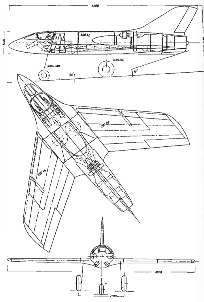
Messerschmitt P1112 S/1 three-view drawing of 27th March 1945.
