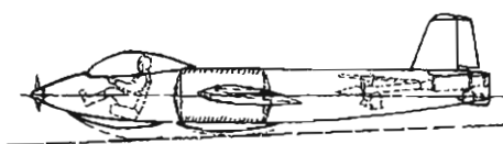
Junkers EF127 'Walli' three-view drawing.
