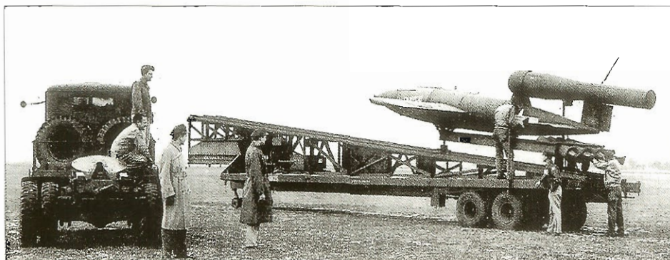
A mobile firing ramp for launching jet-propelled aircraft and missiles, in this instance a US-built copy of the V-1 flying-bomb, accelerated by a battery of four solid-fuel rocket motors.
