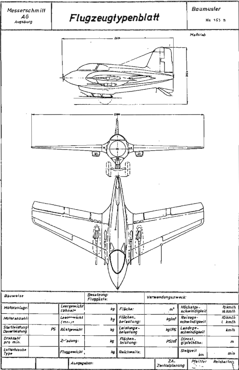
Messerschmitt Me 163B works three-view drawing
