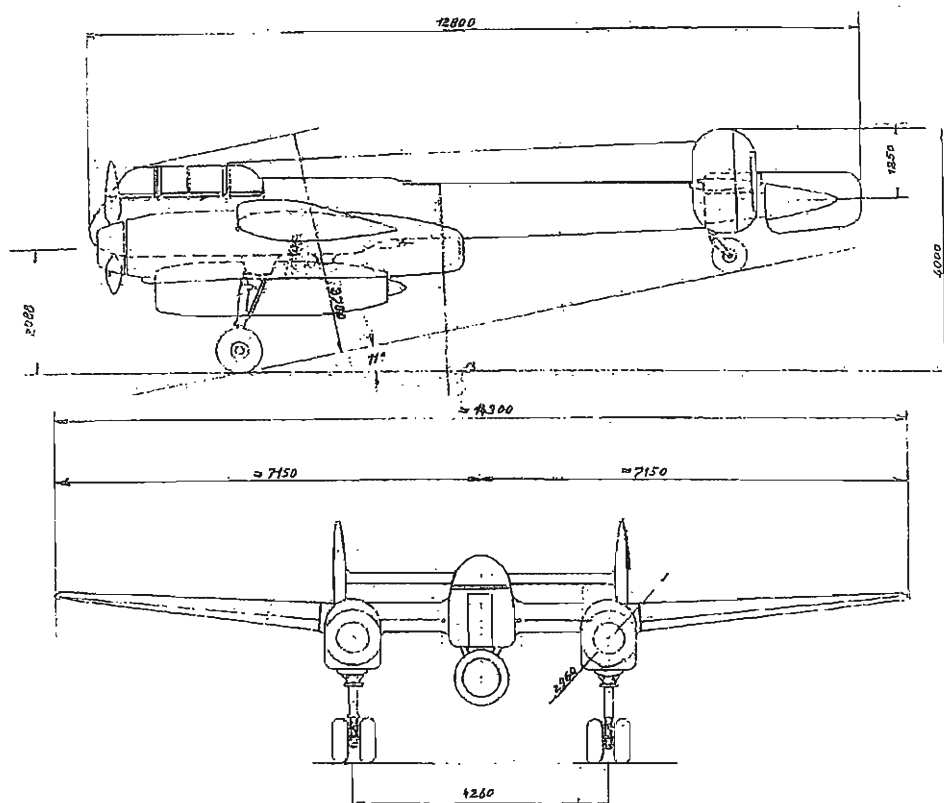
Arado Ar 240A-0 works drawing with dimensions and a Jumo 004 turbojet.
