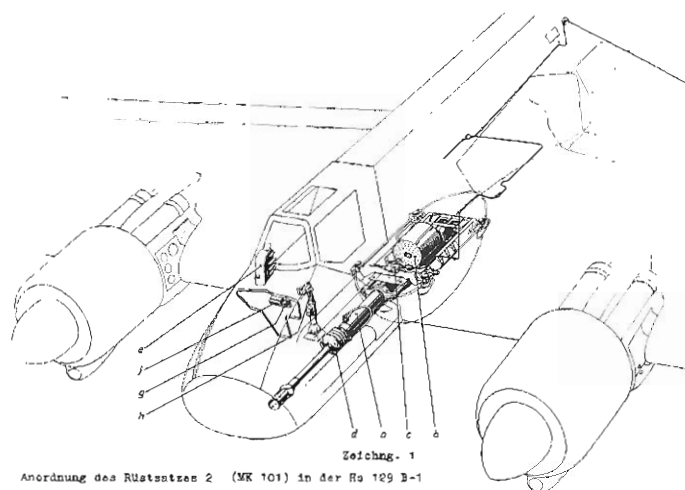
Above: Installation drawing of the Hs 129 with Rüstsatz 2 (one MK101 cannon).
