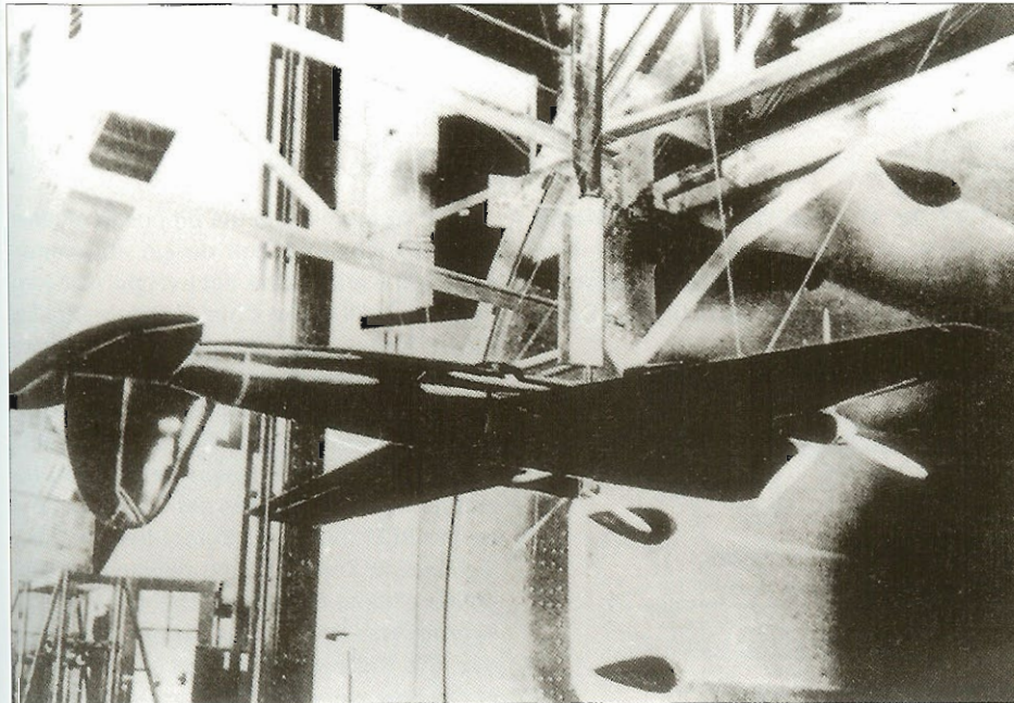
Partial full-size mock-up of the AGO FP-30 (Ao 225).
