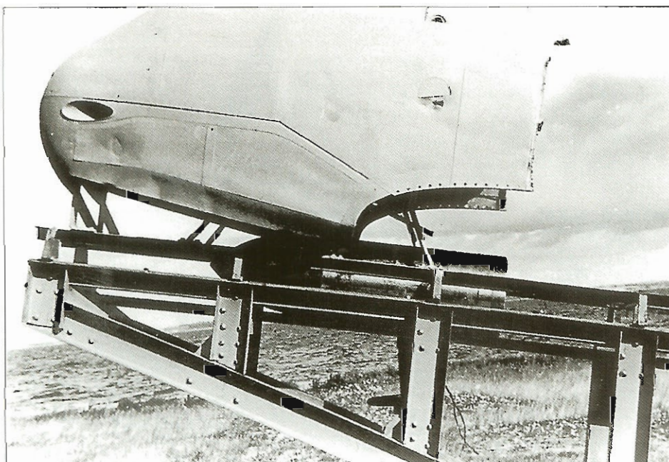
The airborne 'Dicke Berta' (Big Bertha). The heaviest aircraft weapon ever developed, the RZ100 is seen here on an experimental launching ramp beneath the dummy Messerschmitt Me 210 fuselage nose.
