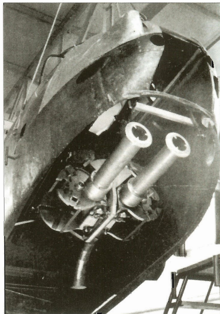
Below: An RZ 65 pair with 8-round magazines.
