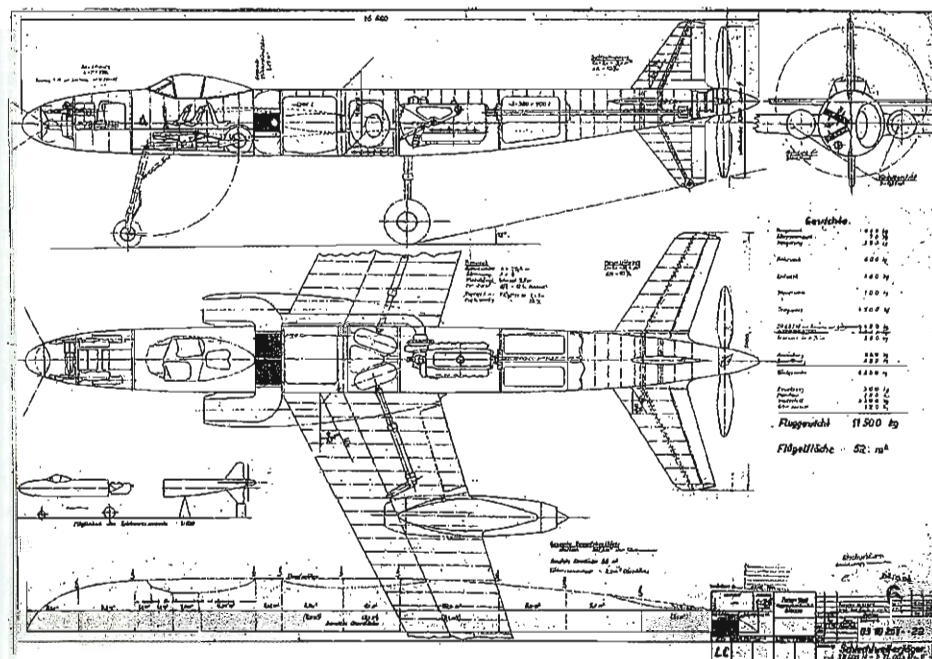
Focke-Wulf 0310251-22 works drawing. The DB 603N drives a single four-bladed propeller and has longer wingroot air intake ducts than the 0310251-13.
