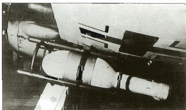
The 28/32cm Wurfkörper as a Bordwaffe (airborne weapon) beneath the port wing of a Focke-Wulf Fw 190A-5/U4.
