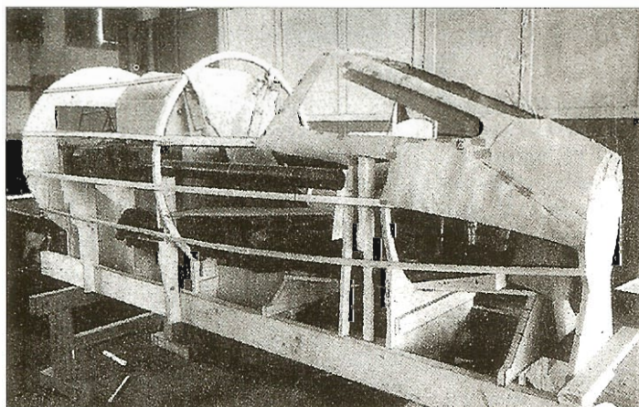
Below left and right: Messerschmitt P1112/V1 mock-up cockpit of March/April 1945.
