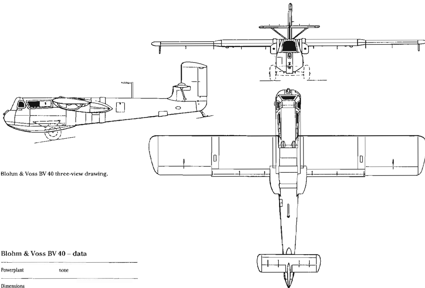
Blohm & Voss BV 40 V1 (PN+UA) port side view.
