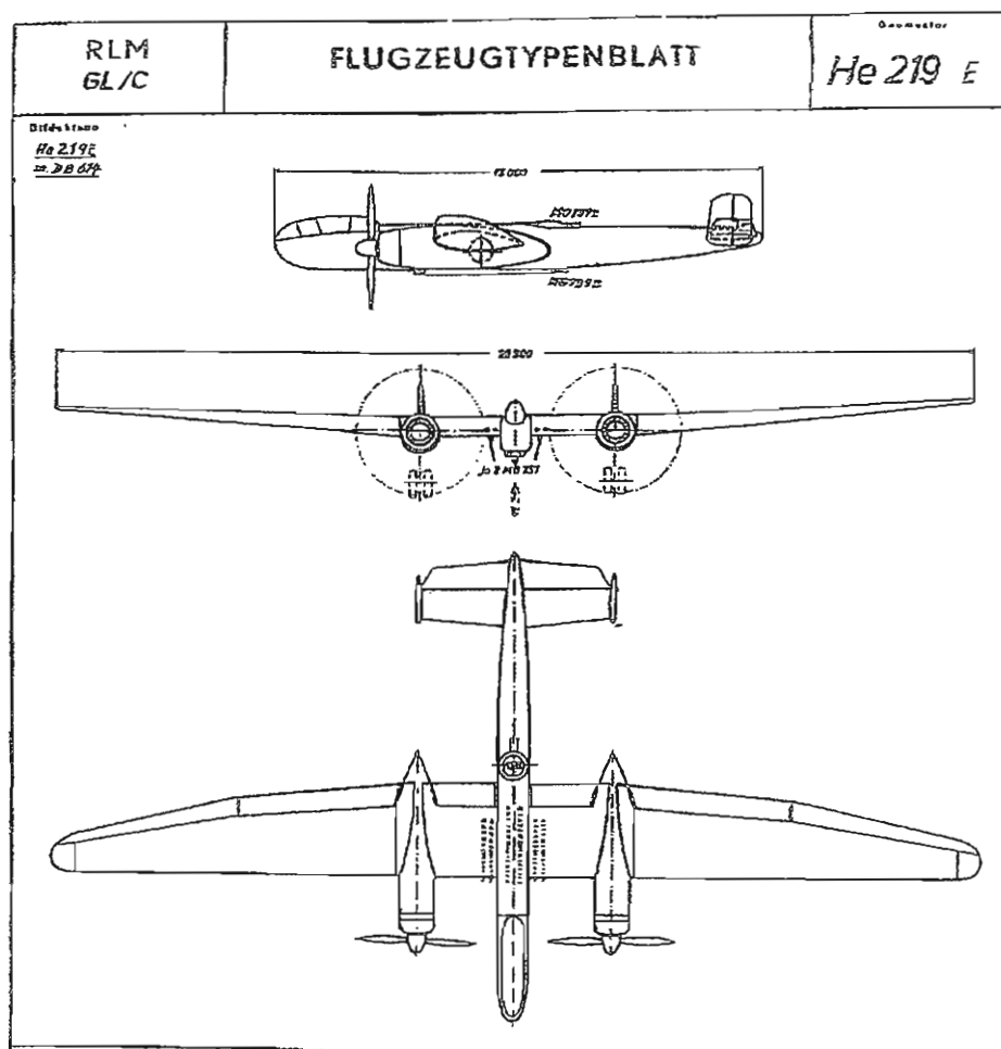
Heinkel He 219E three-view drawing of 7th July 1944 with Hütter wings.
