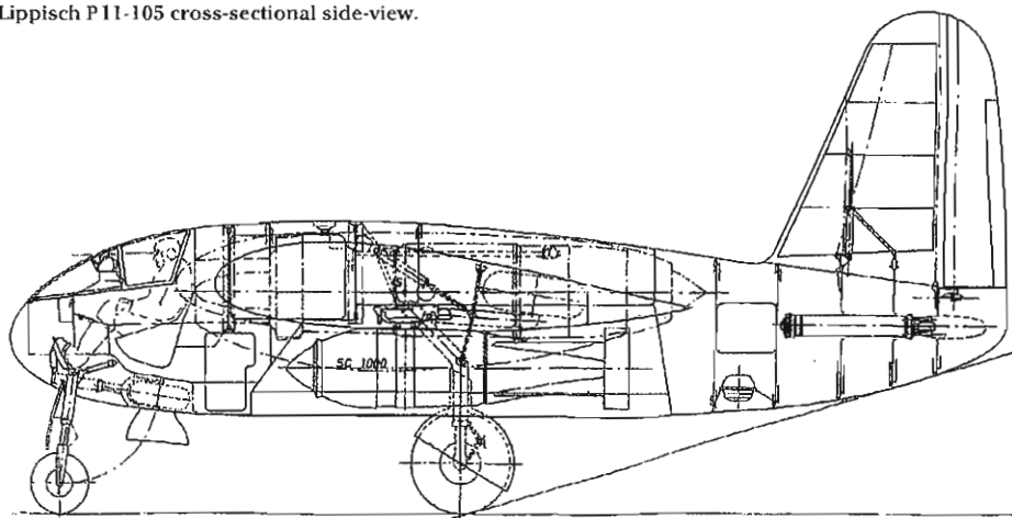
Lippisch P11-105 cross-sectional side-view.
