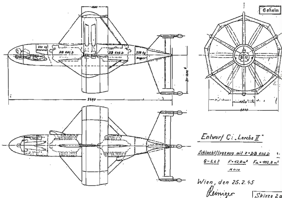
Heinkel 'Lerche II' Entwurf C – drawing dated 25th February 1945.
