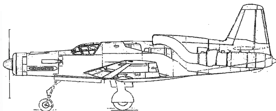
Dornier P 232/3 cross-sectional side-view drawing.
