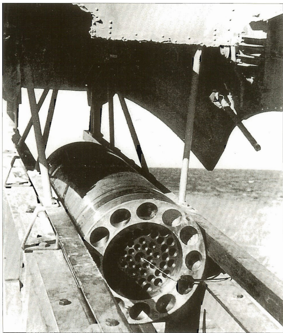
The canted rocket exhaust nozzles provided spin stabilisation for the RZ100.
