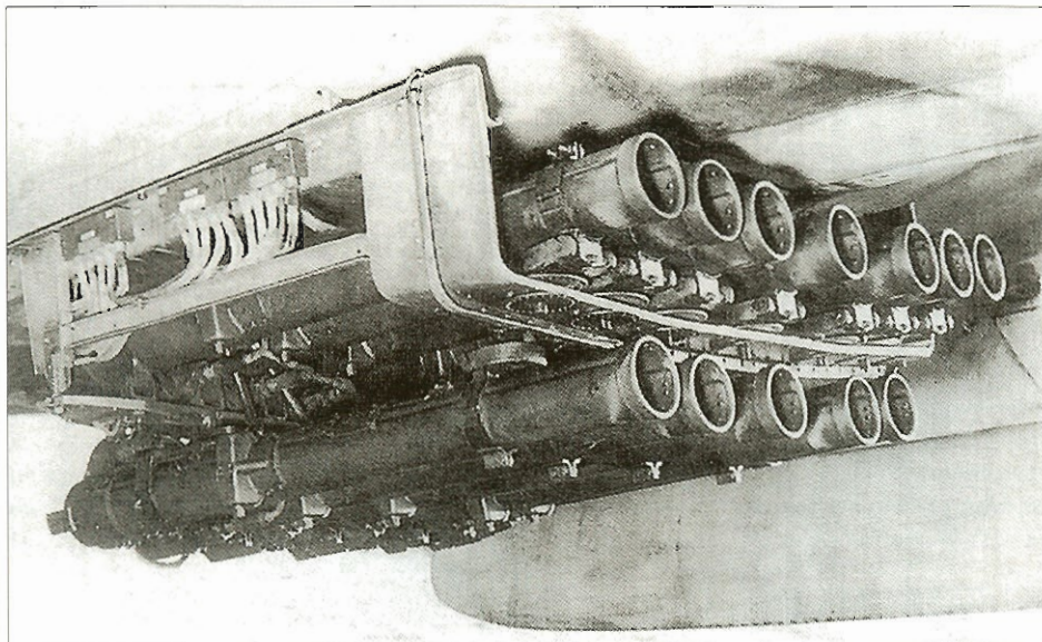
Above: Twelve RZ 65s in two rows beneath an Me 110F-2 fuselage.
