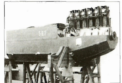
Below: Junkers J 4 armoured trough of 5mm-thick chrome-nickel steel. It weighed 470kg (1,036 lb).
