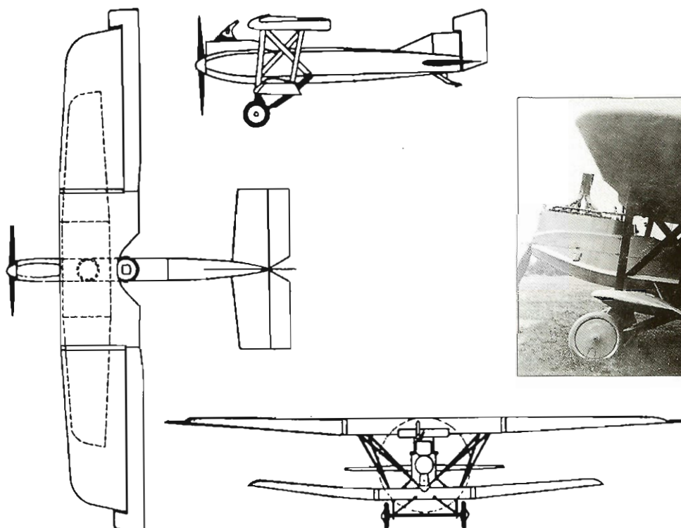
Below: Junkers J 4 with Benz Bz IV motor.
