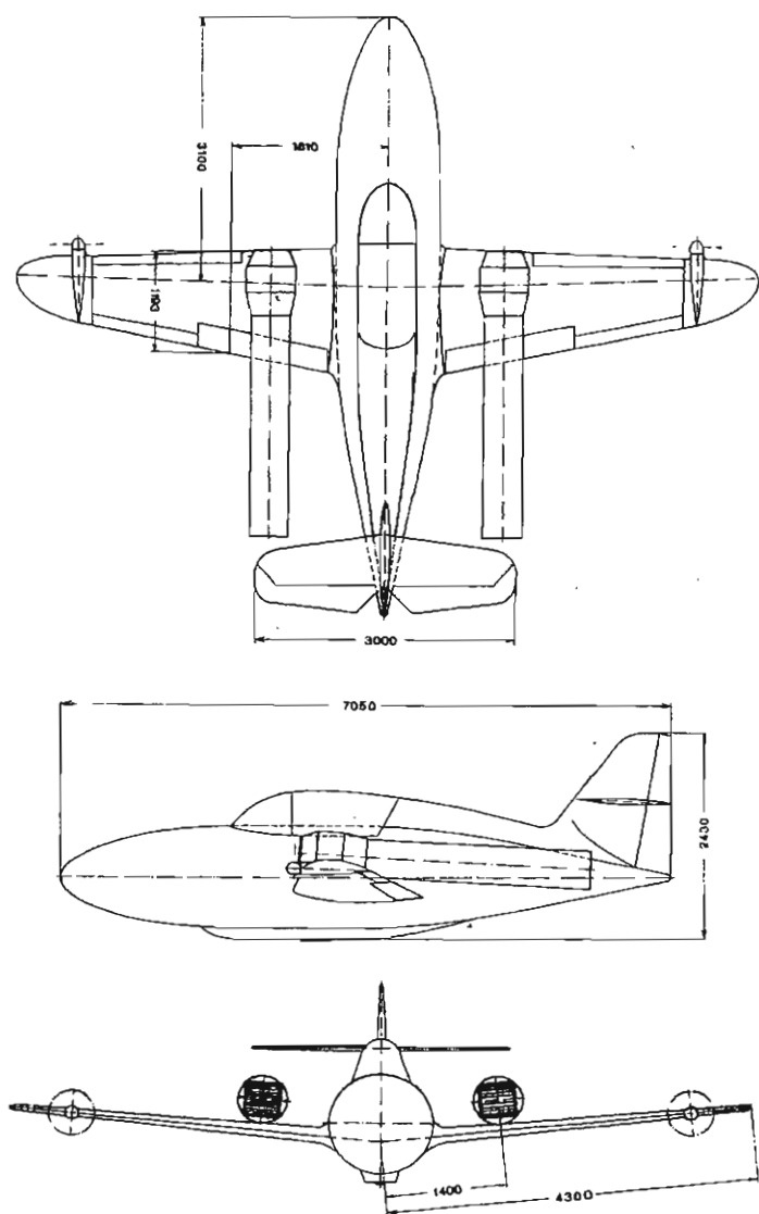
Above: Messerschmitt Me 328B – drawing dated 15th December 1942.
