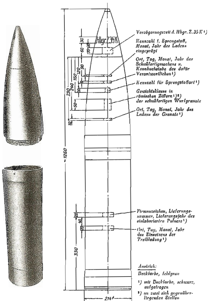
Above: Descriptive drawing of the 21cm Wfr.Gr.42.
