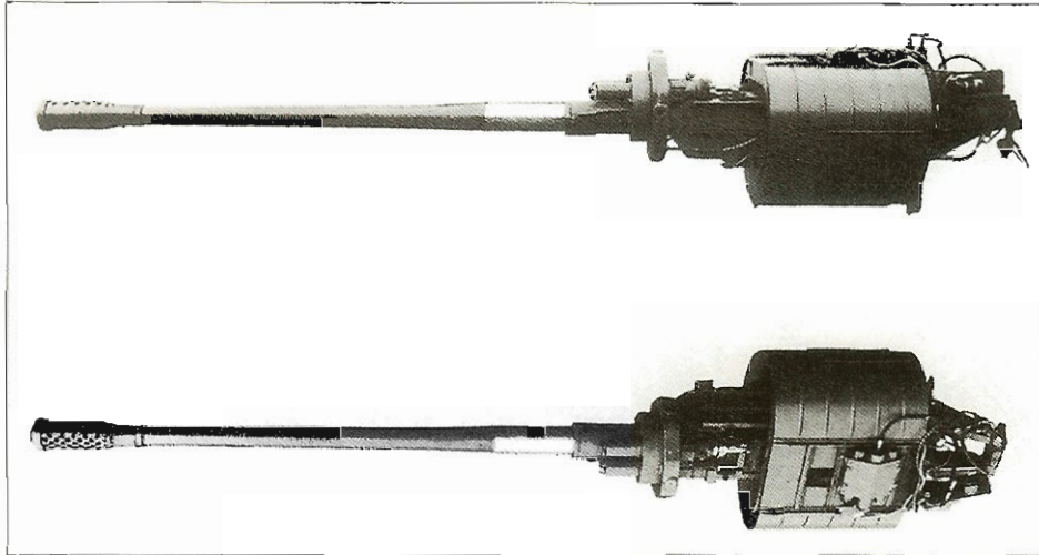
The BK 5 Bordkanone seen from two perspectives.
