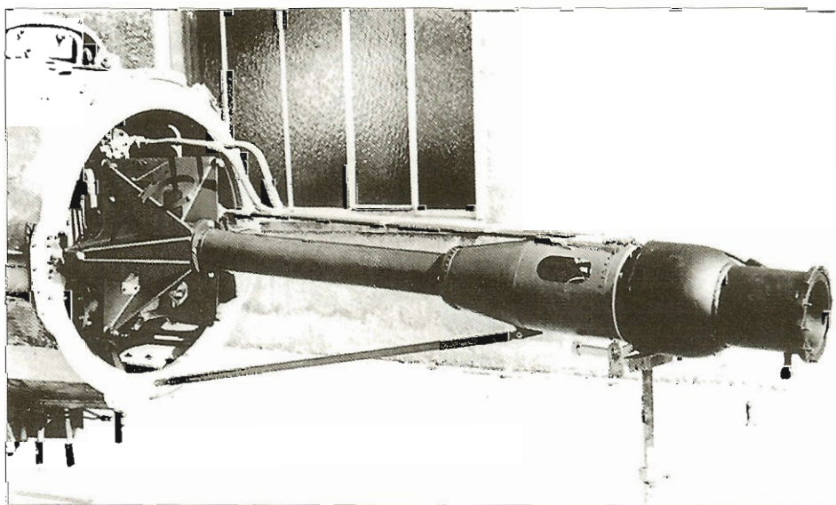
Walter 109-509A-1 rocket motor in the Me 163B.
