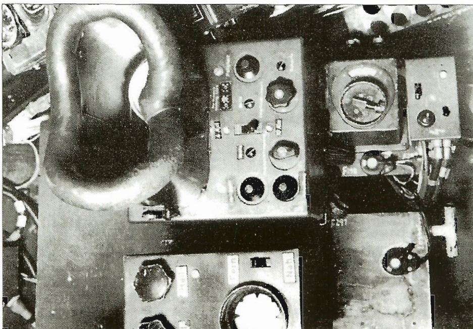
Partial view of the directional, sighting, and control equipment of the German FuG 240 'Berlin 1a' radar.
