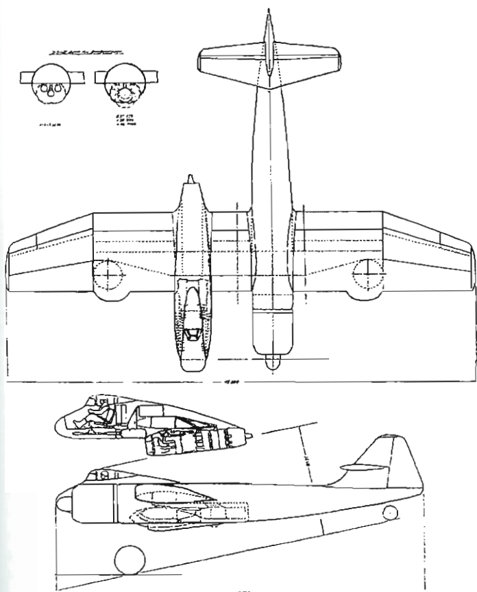
Blohm & Voss P194.01 with one BMW 003A turbojet. The firm's artist inadvertently omitted the empennage surfaces in the head-on view.
