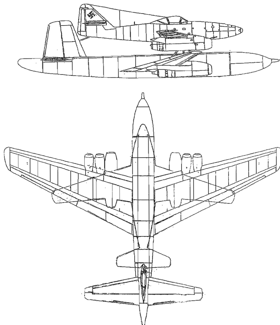
Junkers Ju 287 explosives carrier beneath the Messerschmitt Me 262A.
