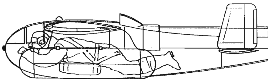
Pilot accommodation in the DFS 'Eber'.
