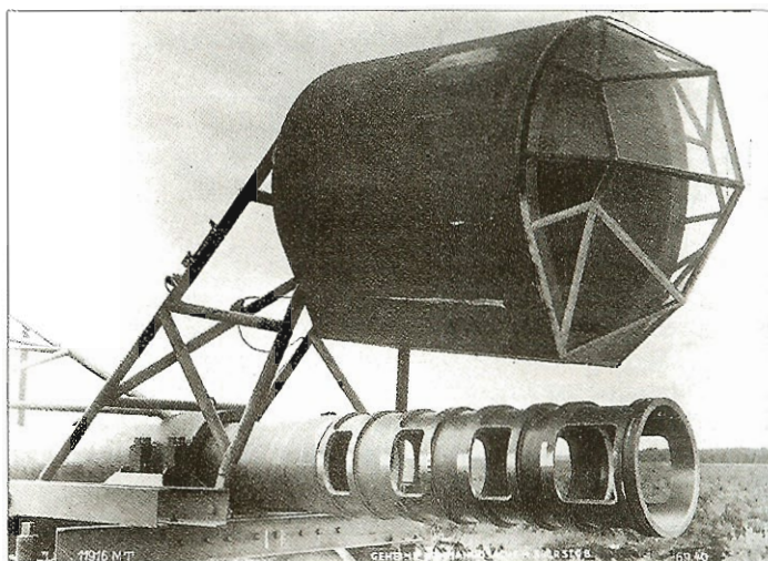
Test arrangement of a mock-up Do 217 nose with the Gerät 104 at the E-Stelle Tarnowitz.
