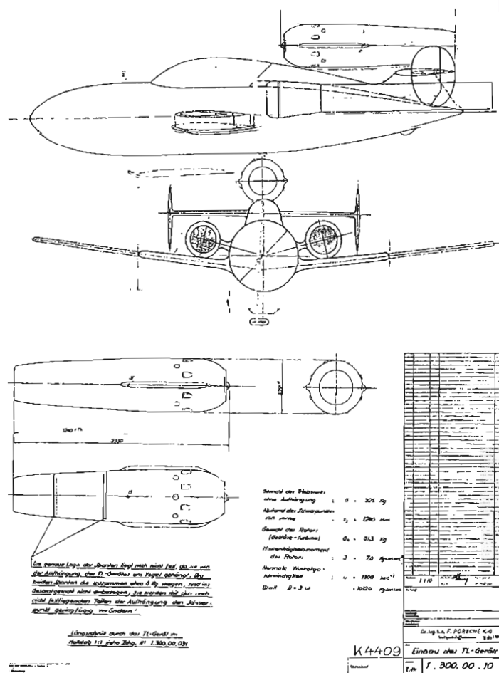
Above: Messerschmitt Me 328 works drawing with two Argus As 014 pulsejets at the fuselage sides, with superimposed dorsally-mounted Porsche 109-005 turbojet. As visible in the head-on view, this Me 328 project study had constant-chord wings of 7.4m (24ft 3/4in) span which could be retracted in flight to only 4m (13ft 1 1/4in) to increase its maximum speed. Overall length was 7.25m (23ft 9 1/4in) and tailplane span 3.2m (10ft 6in), the horizontal tailplane having a leading-edge sweep of 38°.
