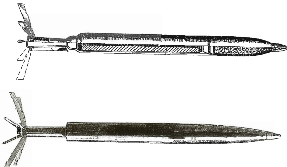
Two views of the R4M with its 8 fins in the folded and extended positions.
