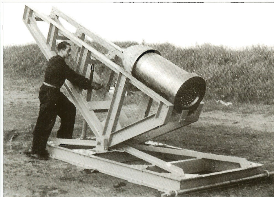
Ground test-firing ramp for the RZ100 in Tarnowitz.
