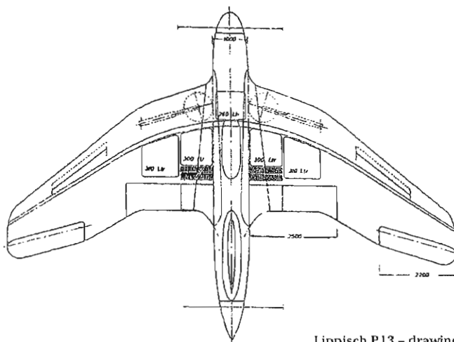
Lippisch P13 – drawing dated 25th November 1942.
