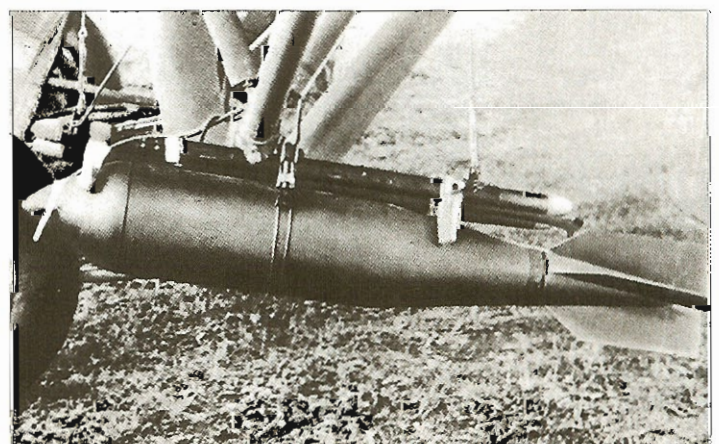
Below right: Suspended bomb on the ETC racks of the Junkers K 47.
