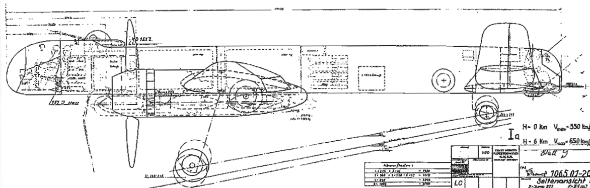
Heinkel P1065.01-20 (Ia) sectional side-view.
