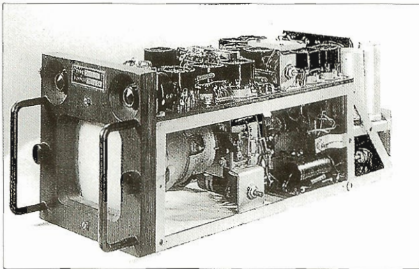
The 'Tonne' television camera and transmitter which captured an image of the target ahead of the guided missile.
