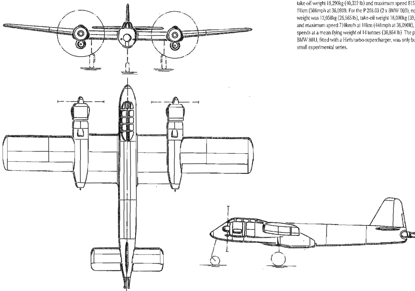
Blohm & Voss P 203.01 three-view drawing.
