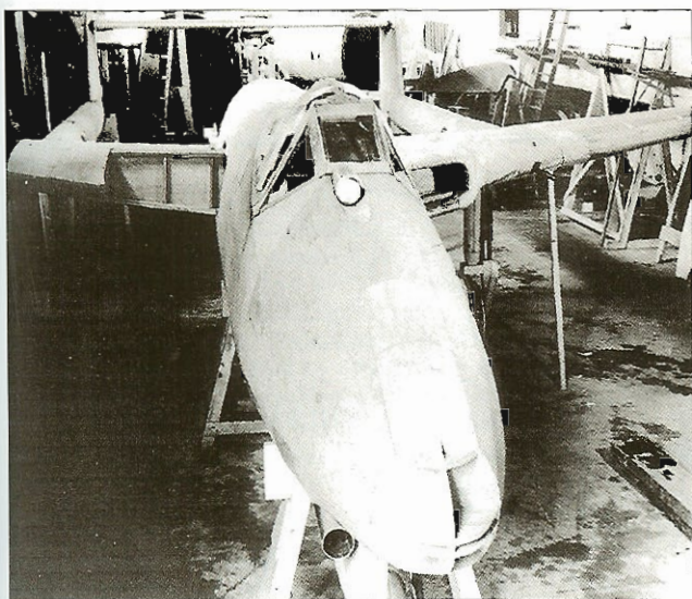
Focke-Wulf P VII full-scale mock-up of 1944.
