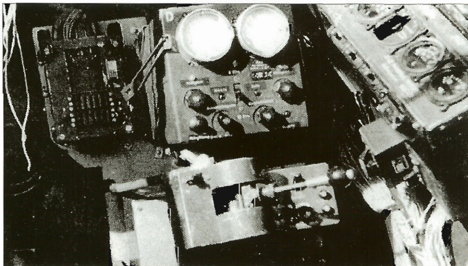
Control console with twin screens for the FuG 240 'Berlin 1a' radar.
