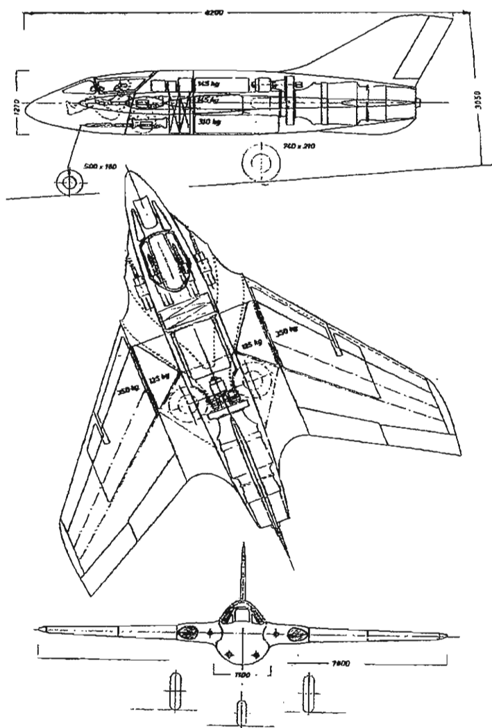
Messerschmitt P1112 S/2 three-view drawing of 3rd March 1945.
