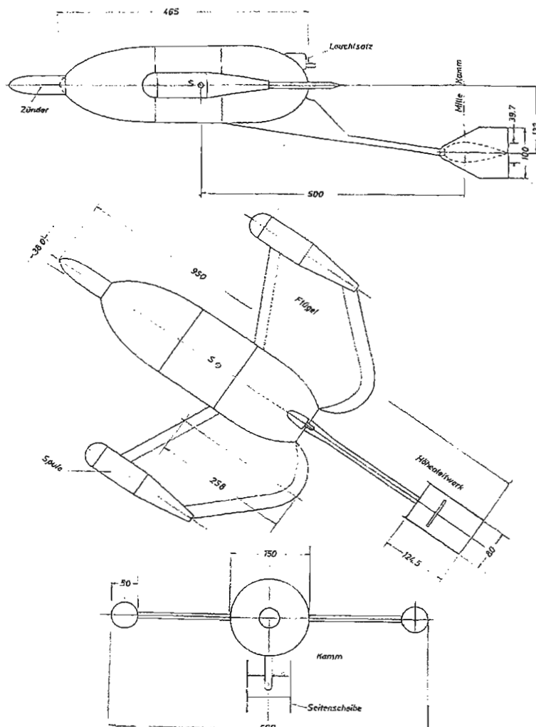
The X7 'Rotkäppchen' missile.
