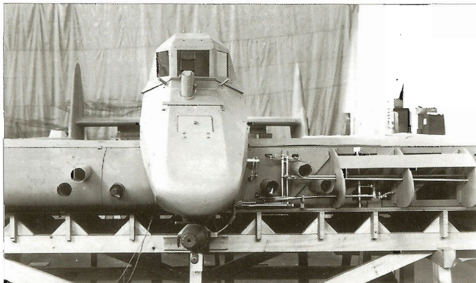
Above left: Focke-Wulf Fw 189 V1b with two-seat armoured crew compartment.
