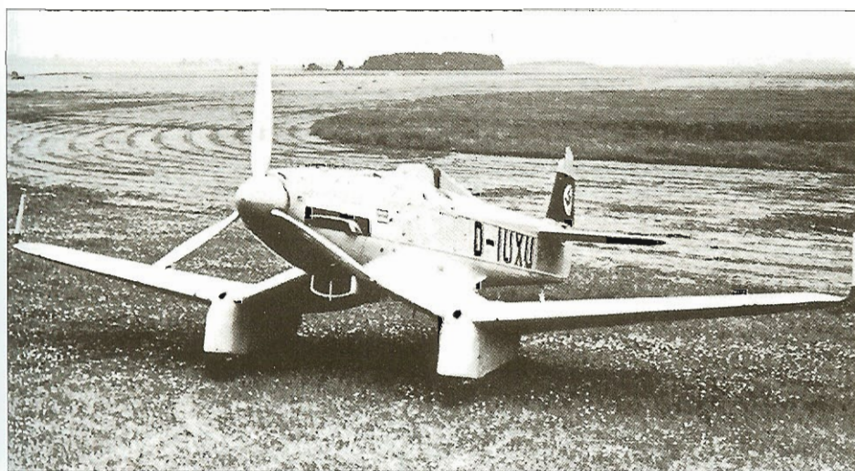
HFB Ha 137 V4 with Junkers-Jumo 210A in-line engine.
