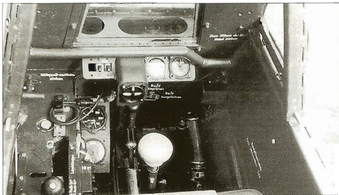
A view of the BV 40 cockpit instruments and controls.
