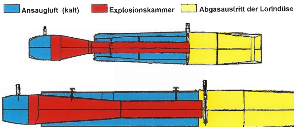
Schematic arrangement of an Argus As 014 or As 044 pulsejet combined with an auxiliary ramjet to increase thrust at high speeds.
