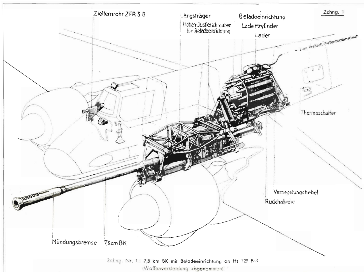
Below: Installation drawing of the Hs 129B-3/Wa with Rüstsatz 3 (one BK7.5 cannon).
