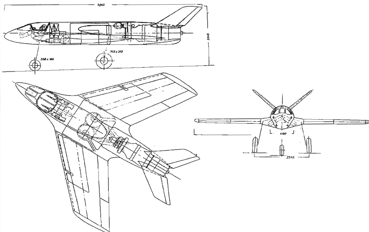
Messerschmitt P1112/V1 three-view drawing of 30th March 1945.
