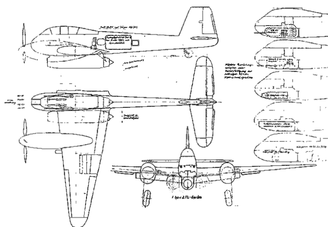
Top: Messerschmitt Me 410B-2 with auxiliary Jumo 004 turbojet.
