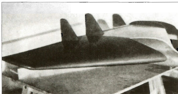
Above left and right: Lippisch P11-121 model photos with wingtips upswept (above) and flat (right).
