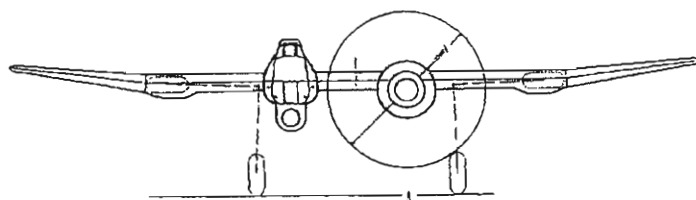
Blohm & Voss P194.01 with one BMW 003A turbojet. The firm's artist inadvertently omitted the empennage surfaces in the head-on view.
