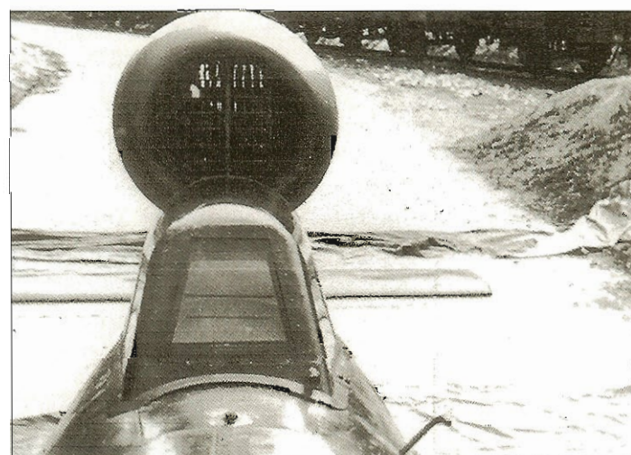
Above: Three views in and outside the cockpit of the Fi 103Re-4 'Reichenberg'.
