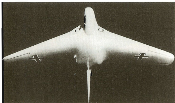
Top and above: Lippisch P11-105 model showing the fixed outboard wing leading-edge slots, trailing-edge controls and the rectangular extendable tail surfaces outlined on the fin.
