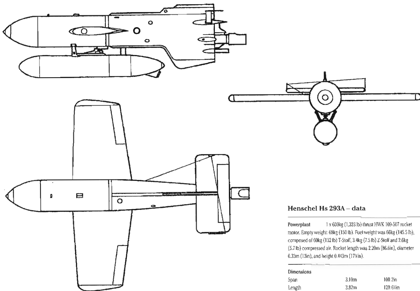
Henschel Hs 293 three-view drawing.
