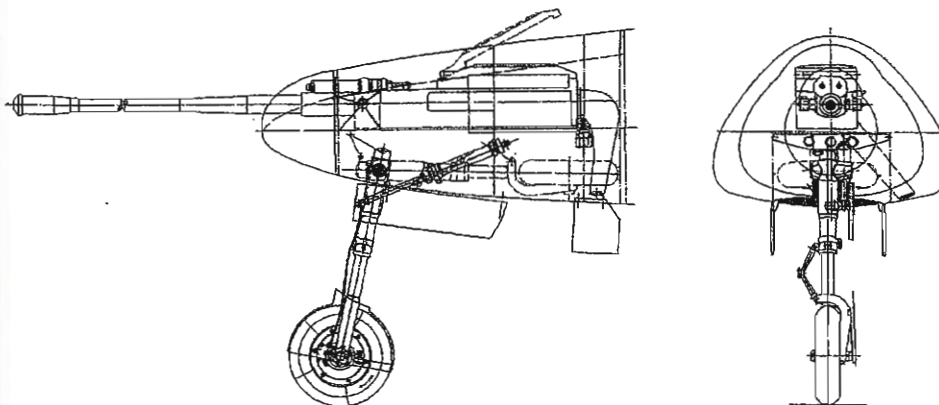
Cross-sectional arrangement of the BK 5 in the Me 410.
