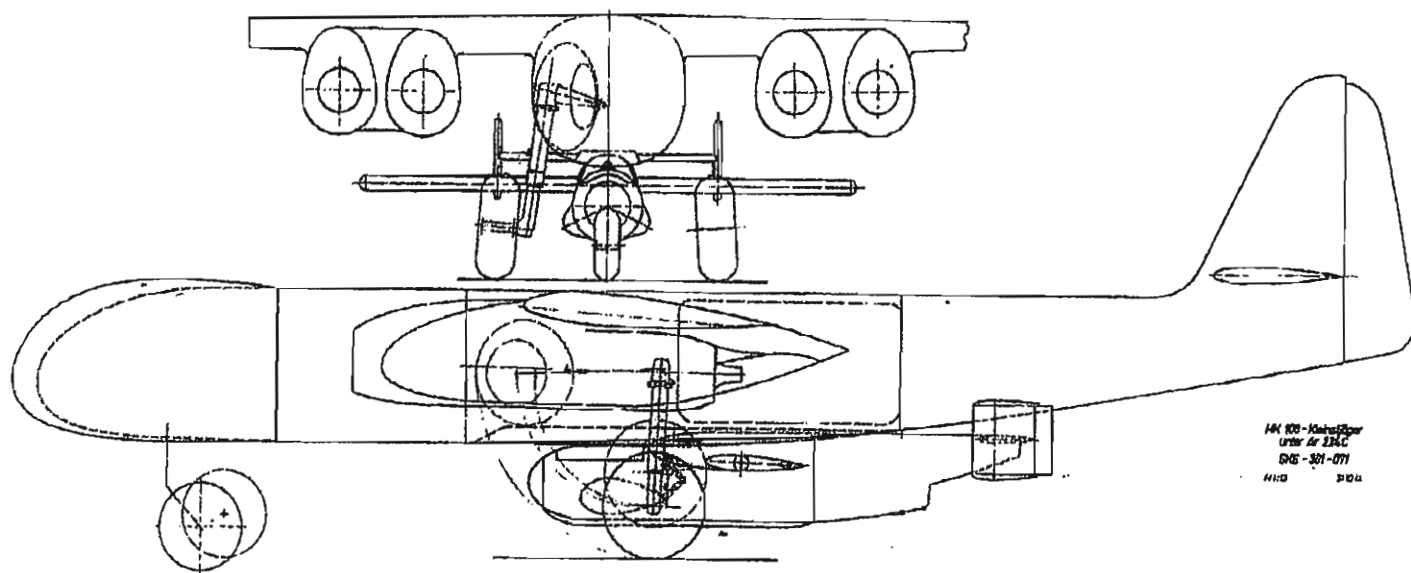
Arado E 381 beneath the Ar 234C-3. Works drawing of 31st October 1944.
