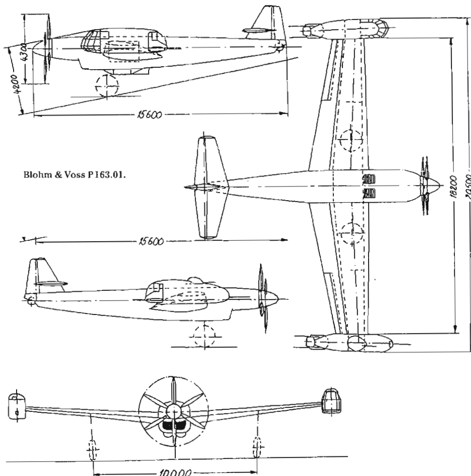
Below: Blohm & Voss P 163.02 with BMW 803.
