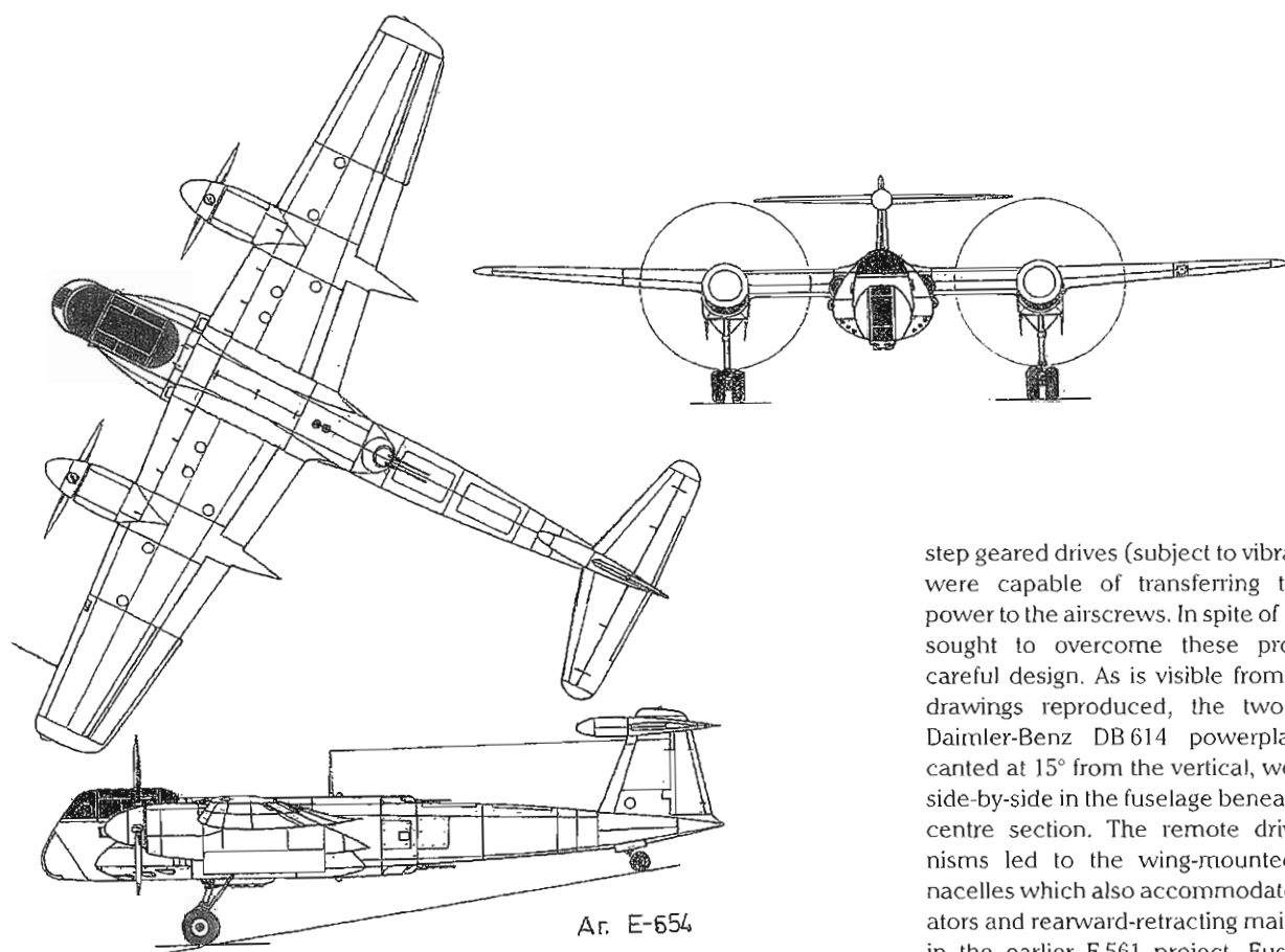
Above: Arado E 654 heavy fighter and ground attack aircraft.
