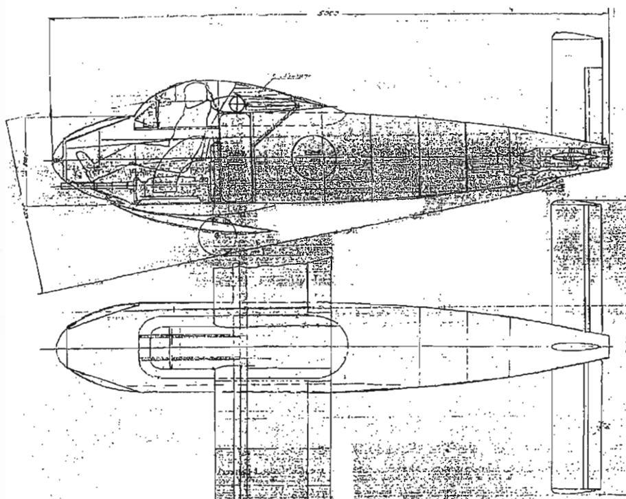
Top: Messerschmitt P1104 Bordjäger works drawing (XII-283) of 12th September 1944.
