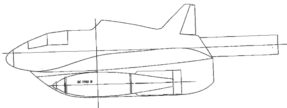
Messerschmitt P 1079/10c variant with streamlined bomb enclosure.
