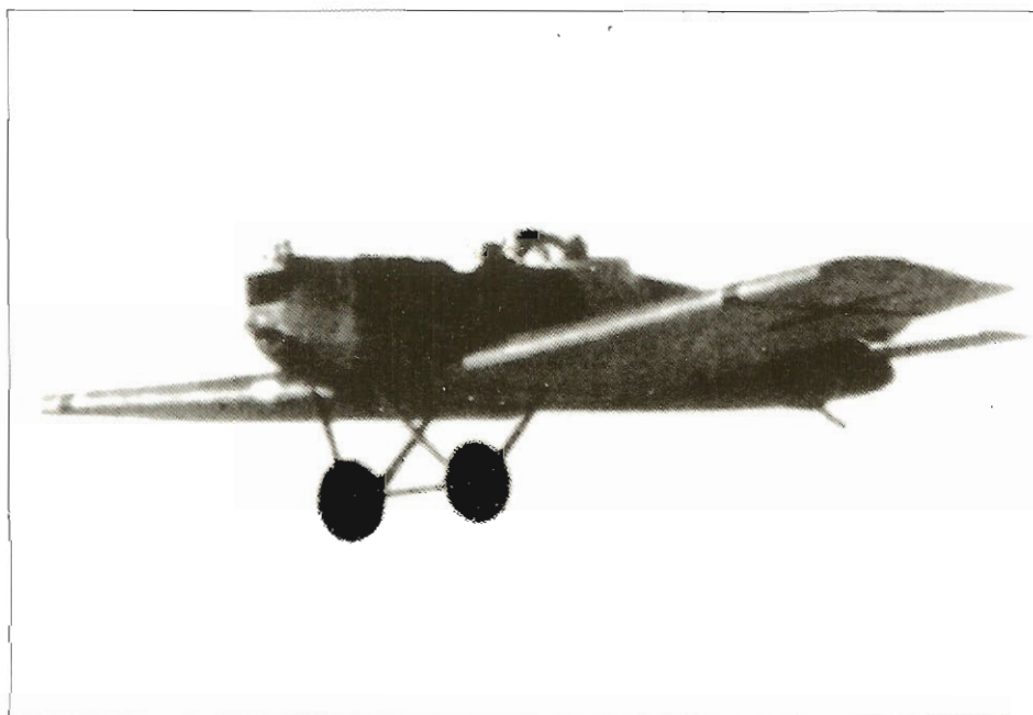
Above: The Junkers J10, photographed here on 19th June 1918, was not only an extraordinary ground attack aircraft but was also the world's first all-metal combat aircraft.
