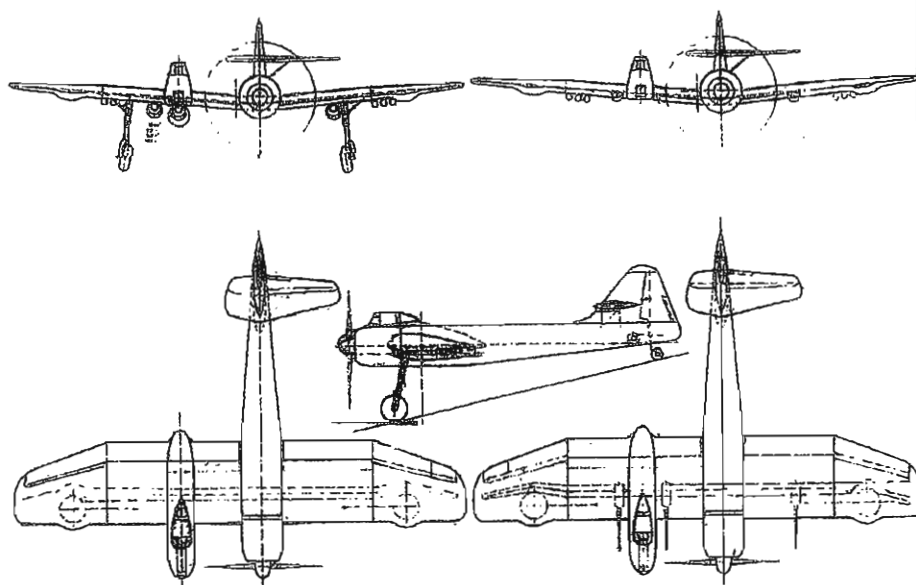
Blohm & Voss BV 237 as Stuka (left) and Ground Attack aircraft (right).
