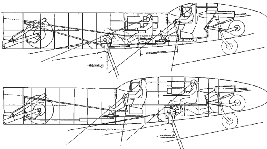
Blohm & Voss P170.01 crew seating proposals.
