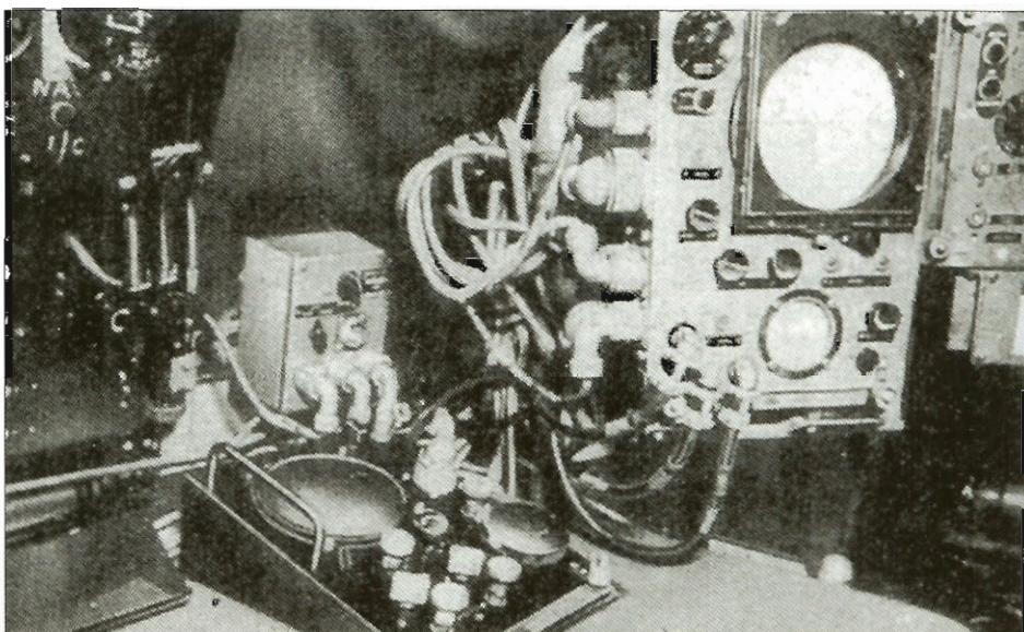
The British H2S centimetre-wave panoramic radar equipment.
