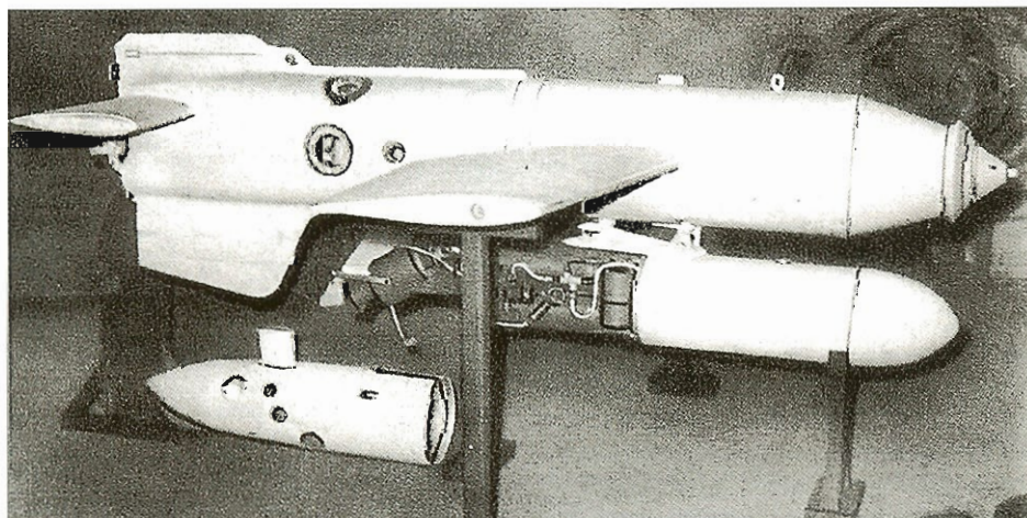
Henschel Hs 293 missile with its Walter 109-507 rocket motor partially uncovered.
