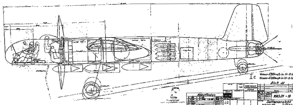
Heinkel P 1065.01-19 (Ic) sectional side-view.
