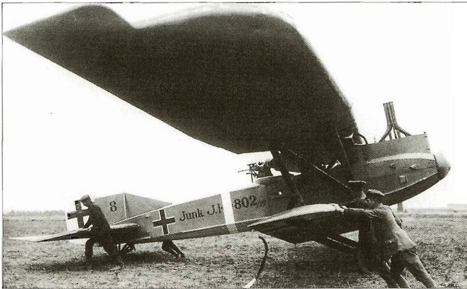
Left: Junkers J 4 with 200hp Benz Bz IV motor and vertical exhaust stacks. Photo dated 3rd May 1918.
