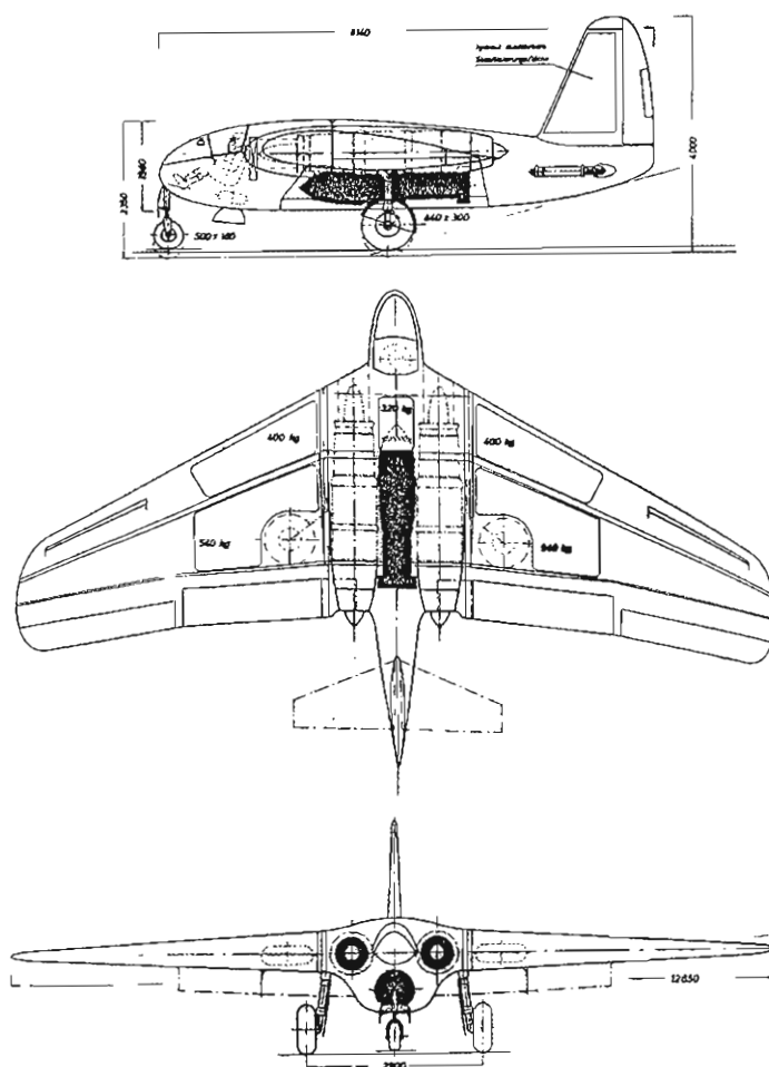
Above: Lippisch P11-105 – drawing dated of 2nd December 1942.
